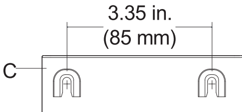
Mounting Template
